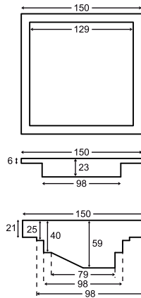
Floor Trap with/without Anti Cockrach Trap
