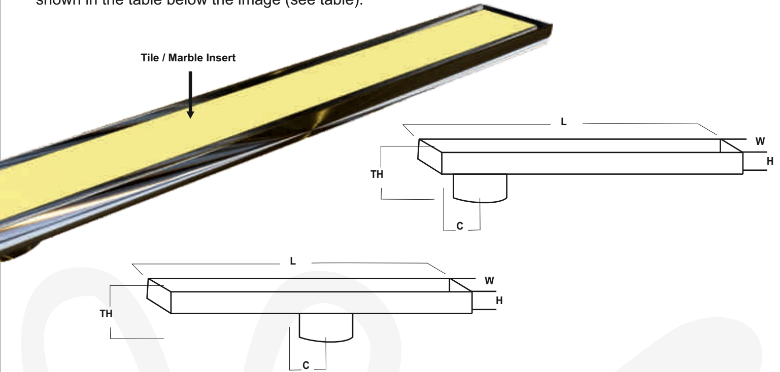
Tile Insert Shower Drain Channels : Available Sizes
